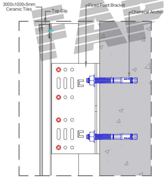
Detail 1 SCALE 1:4
