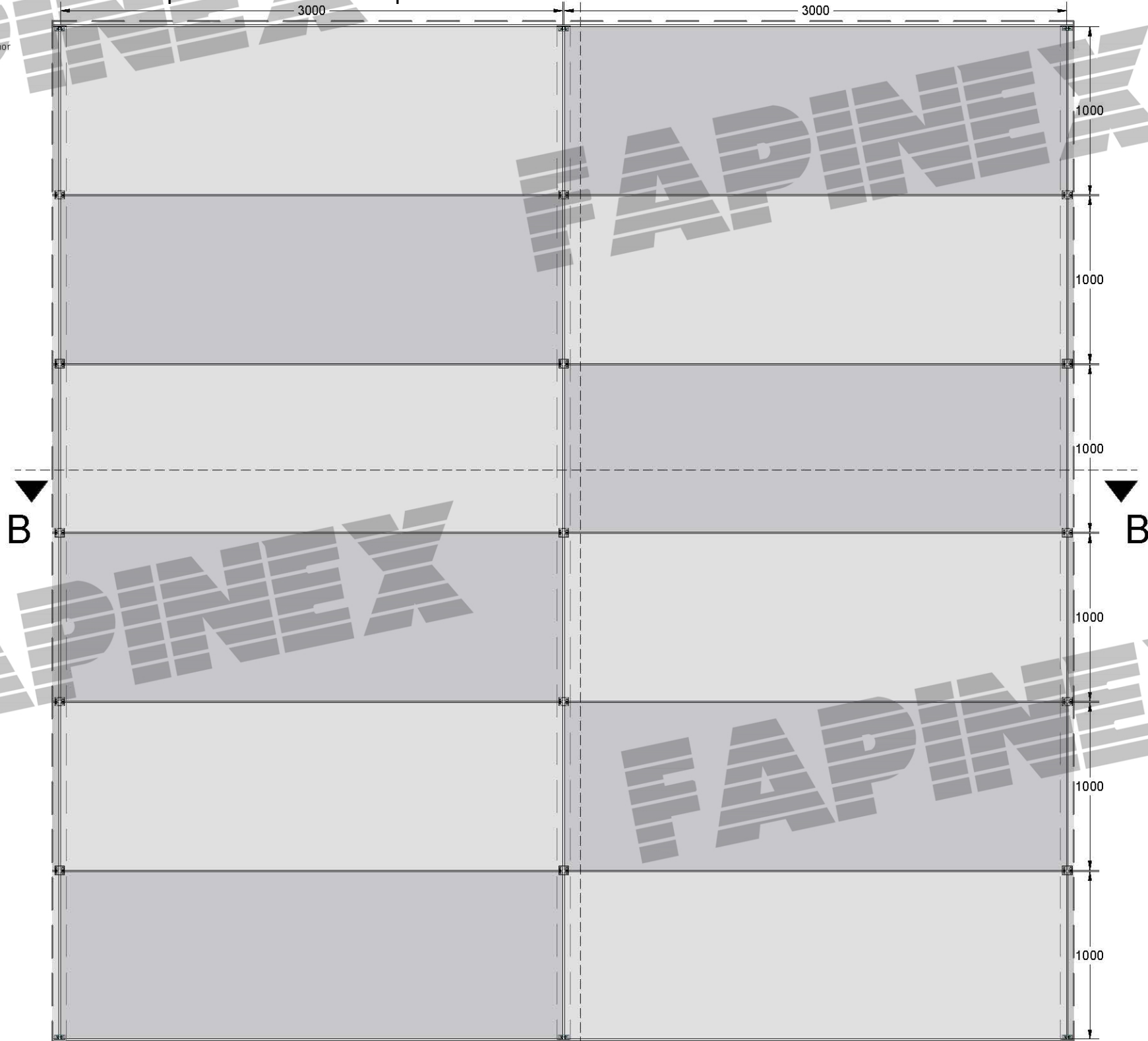
ELEVATION SCALE 1:30
