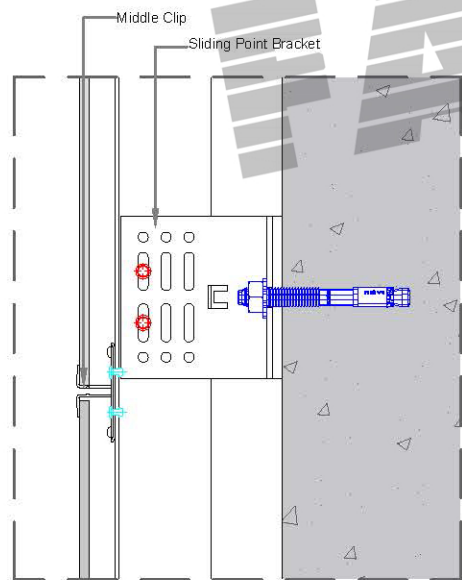
Detail 2 SCALE 1:4
